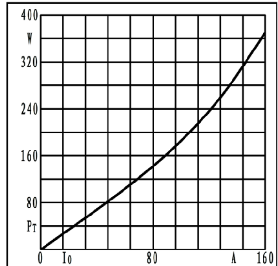
Fig2. Power dissipation
