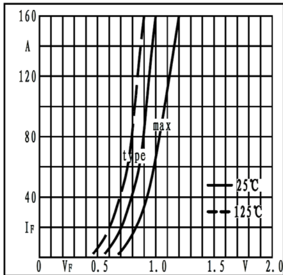
Fig1. Forward characteristics
