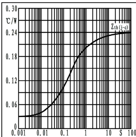
Fig3. Transient thermal impedance
