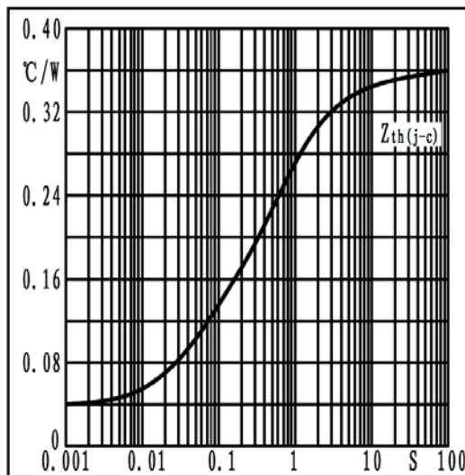
Fig3. Transient thermal impedance
