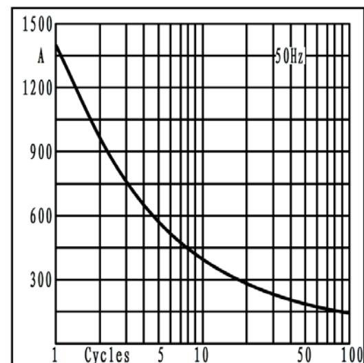
Fig4. Max non-repetitive forward surge current
