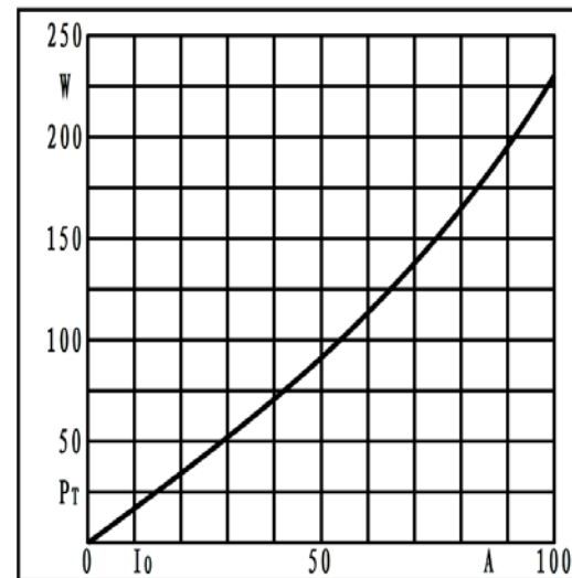
Fig2. Power dissipation
