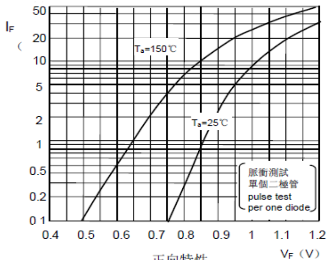
Forward Characteristics
